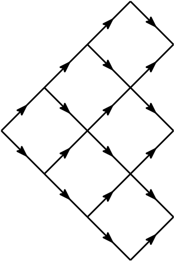
polynomial growth
